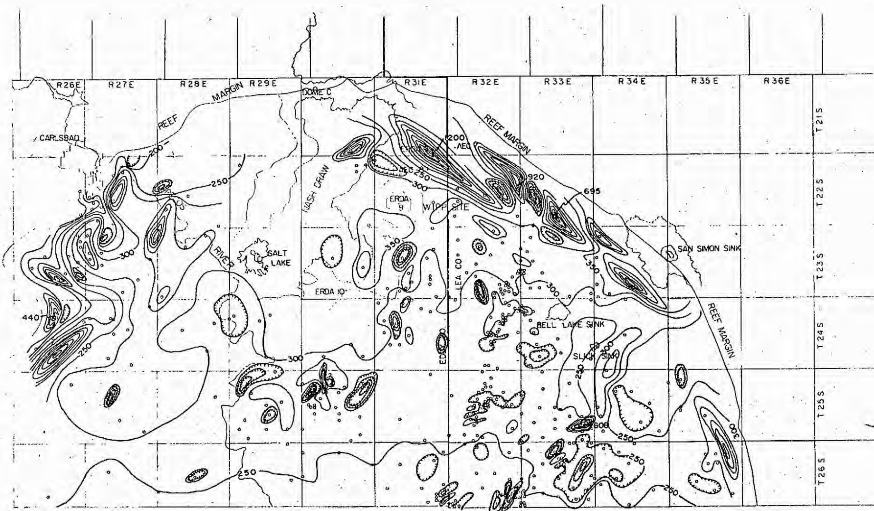
Figure 4. HALITE I ISOPACH
