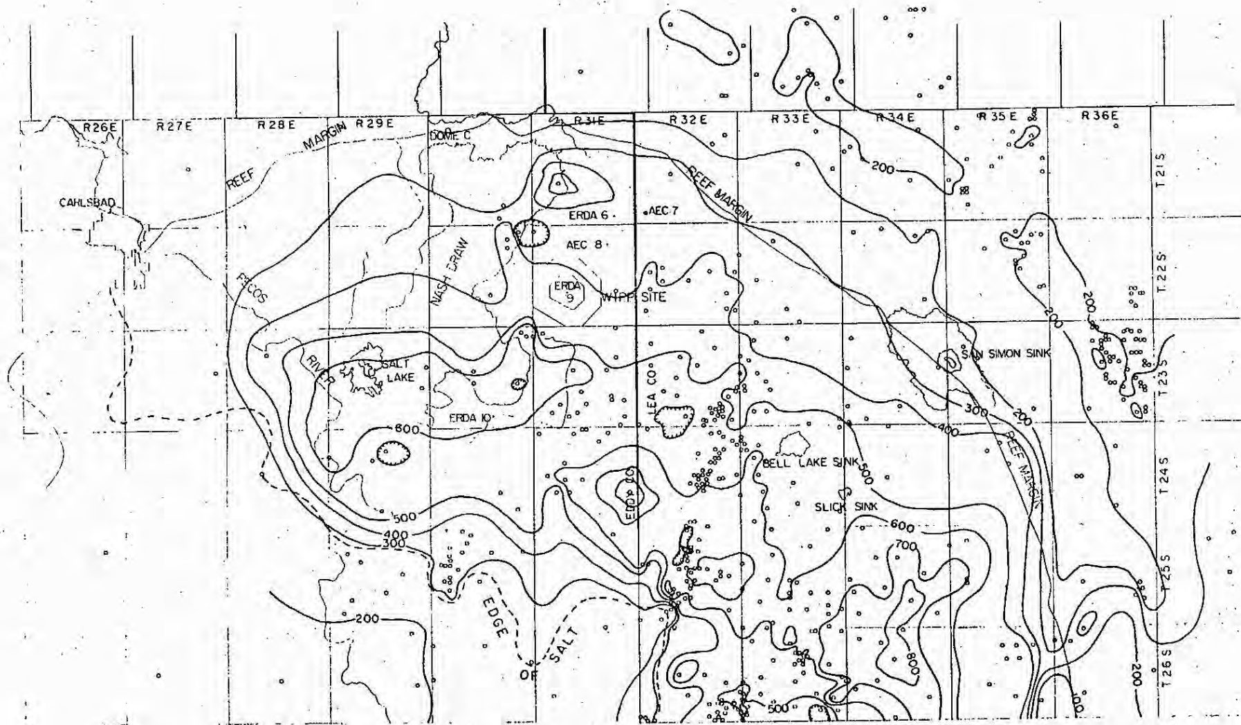
FIG. 8 LOWER SALADO ISOPACH
